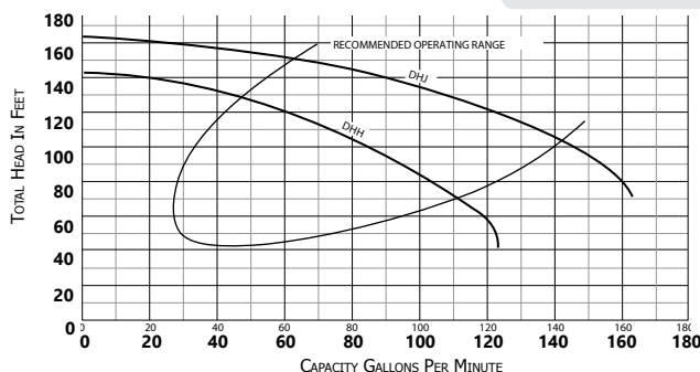
PERFORMANCE CURVES
