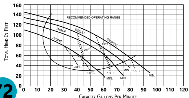
PERFORMANCE CURVES
