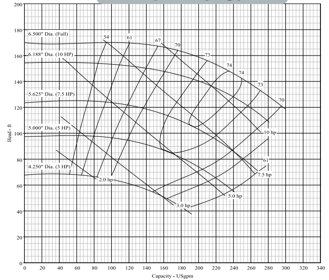
PERFORMANCE CURVE
