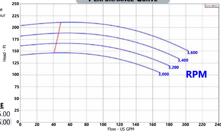
PERFORMANCE CURVE
