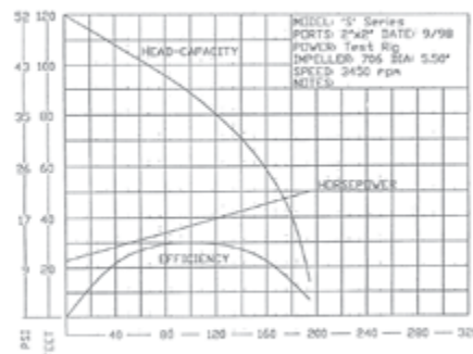
5 HP Pump Curve PERFORMANCE CURVE
