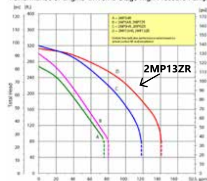
Performance of Engine-Driven 2-Stage High Pressure Pumps
