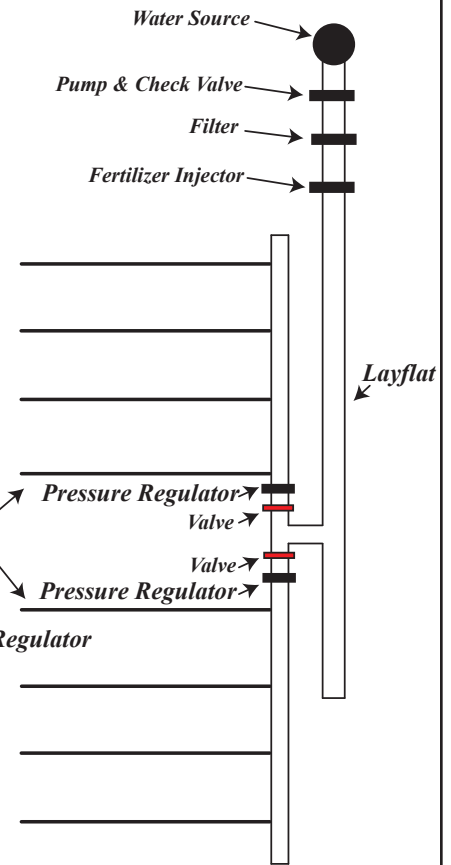
Drip Layout 2
